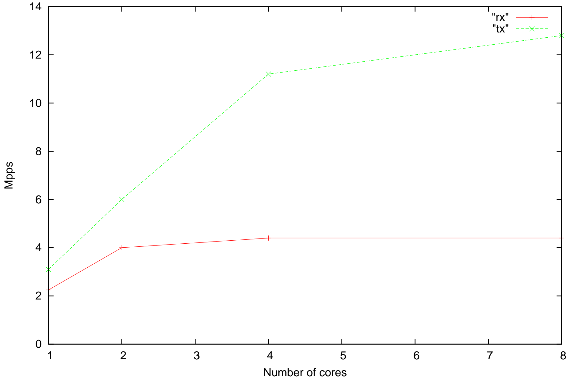
AMD rx and tx dma performance
